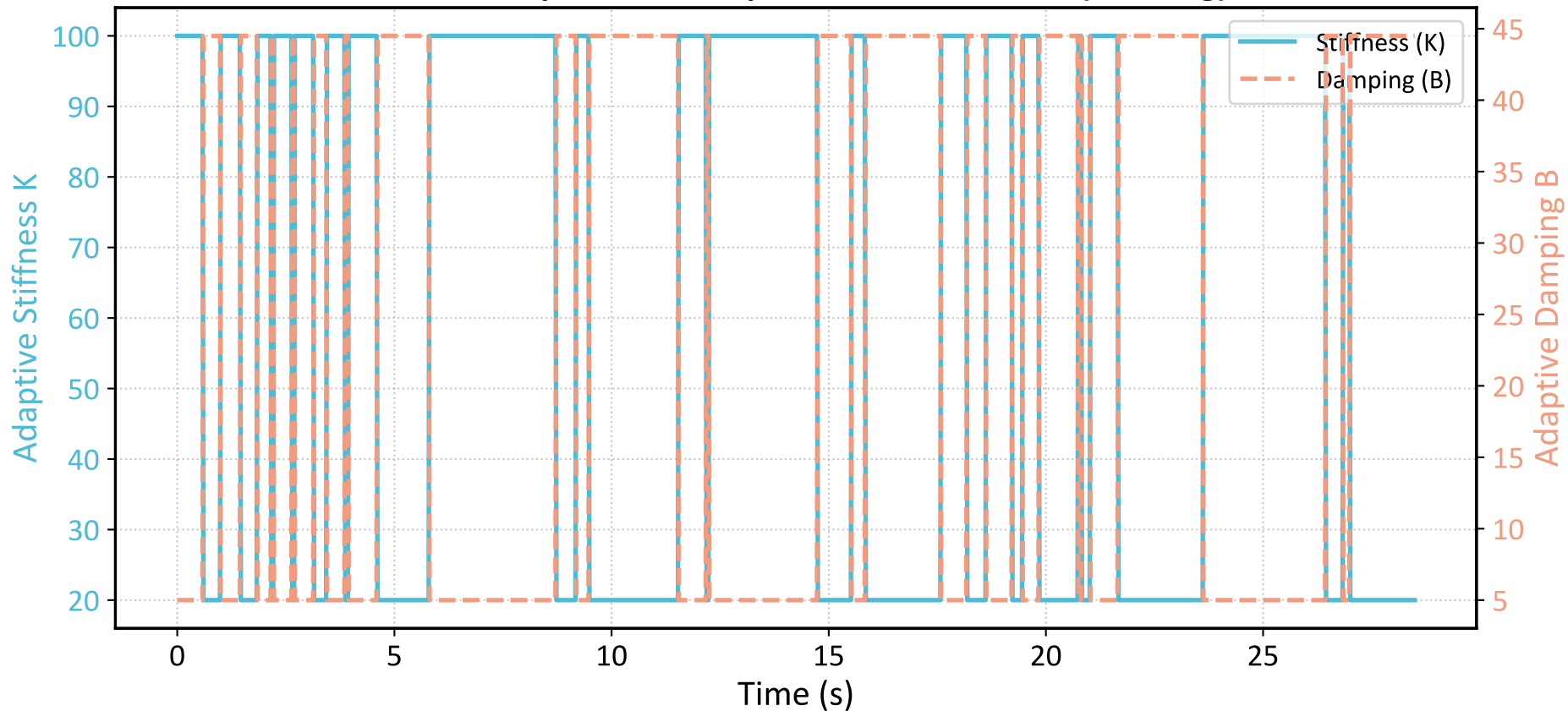
Online Adaptation of Impedance Parameters (Twirling)
